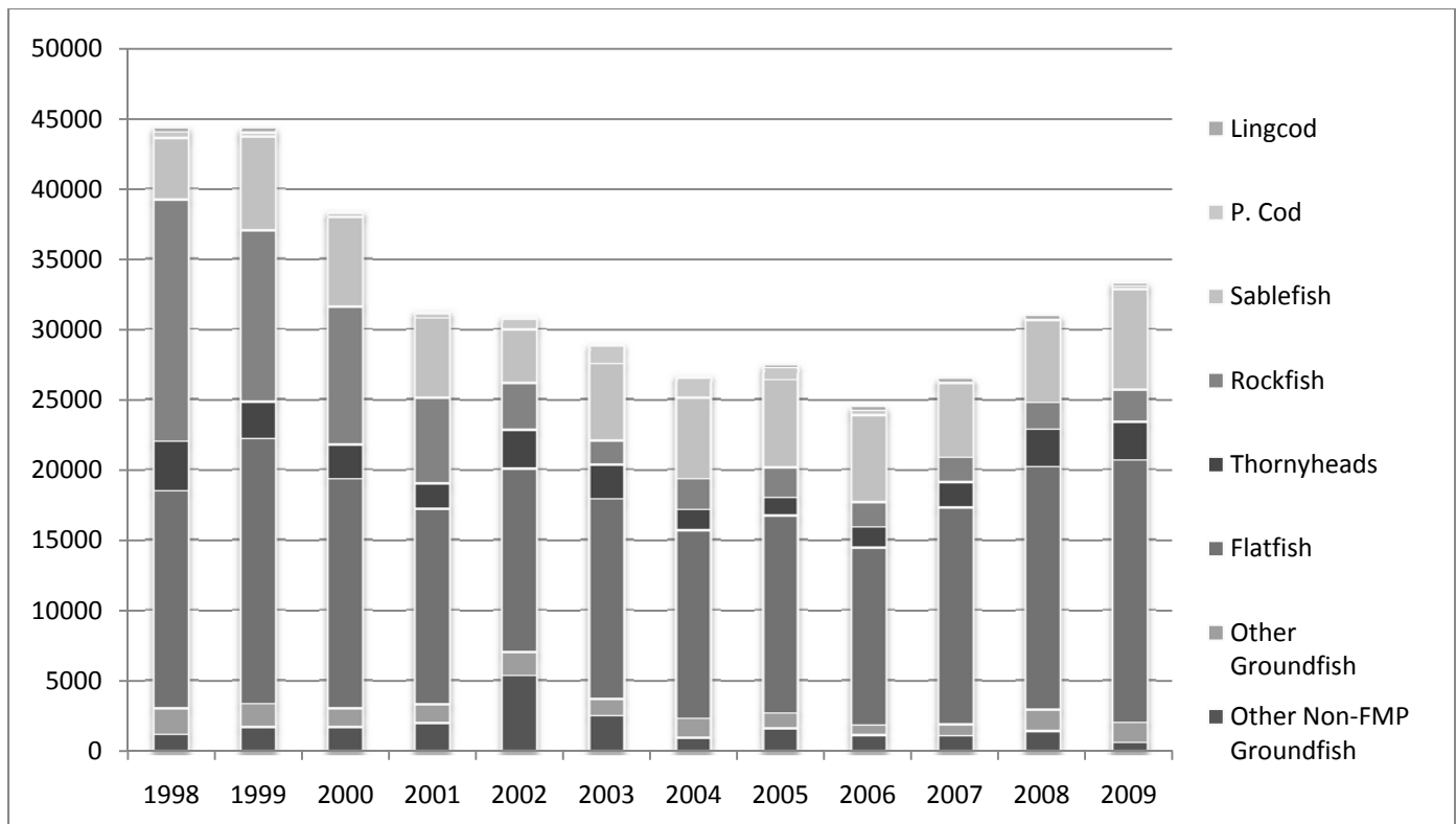
Figure F-2. Nonwhiting groundfish landings (mt), 1998-2009.
