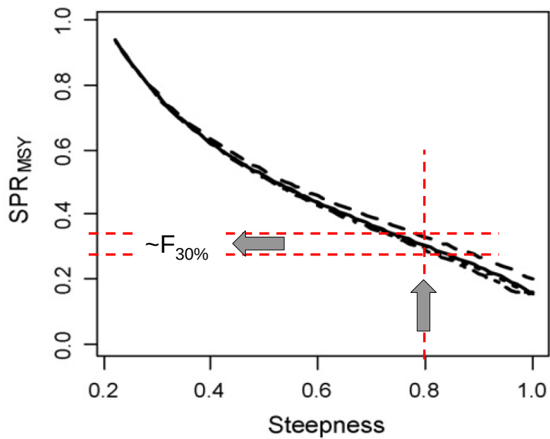
Figure 4-18. Relationship between spawner-recruit steepness ( h ) and the fishing mortality rate, expressed as spawning potential ratio (SPR), that maximizes sustainable yield among four west coast groundfish stocks (taken from (Punt, et al. 2008)).
