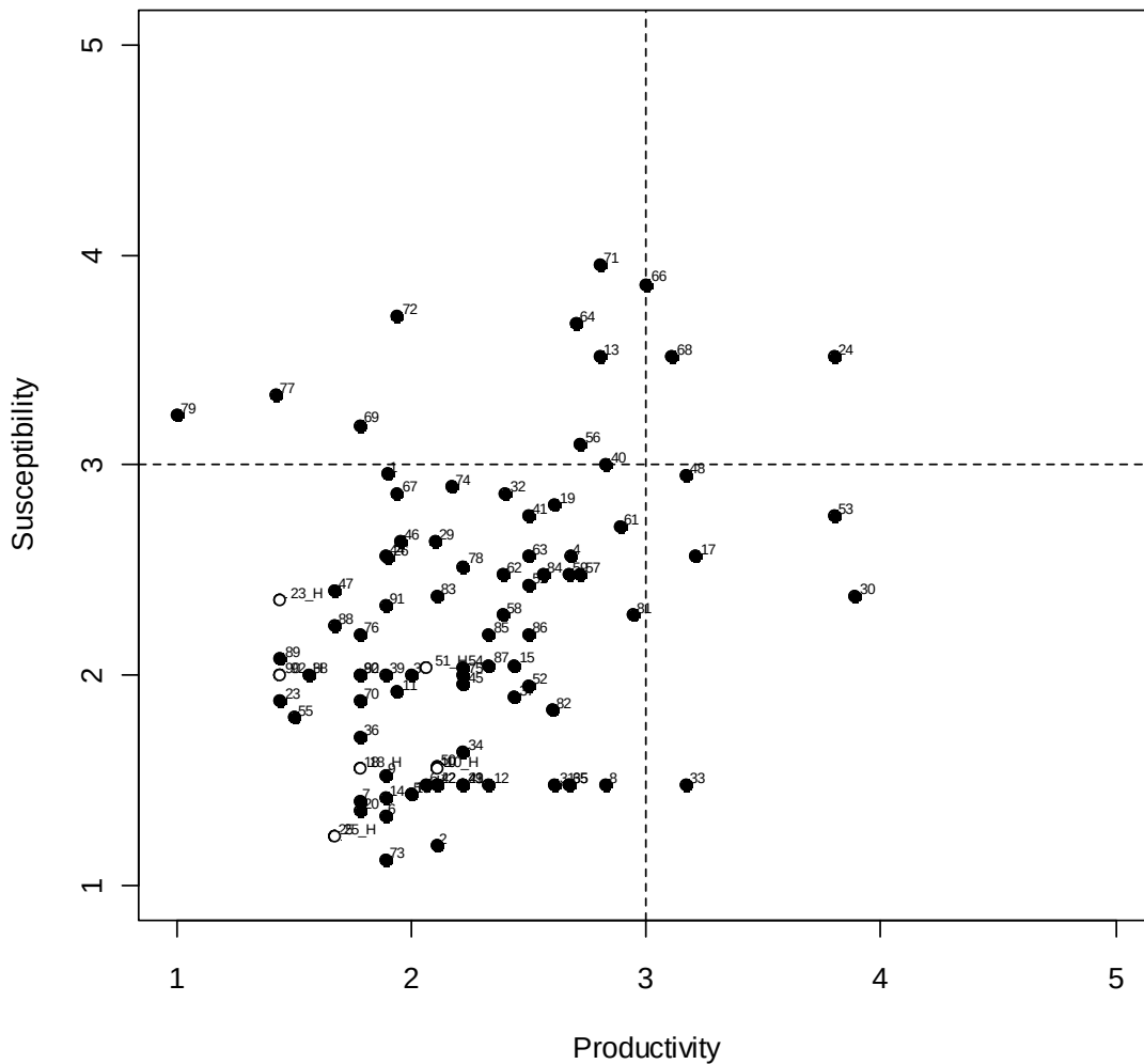
Figure 4-2. Data quality plots for the productivity and susceptibility scores in the PSA for each species (represented numerically in Table 4-4 and Table 4-5) in the west coast groundfish FMP. Higher scores indicate less data quality. Vertical and horizontal lines provide a general guide to relative data quality with values above 3 on either axis considered data poor.
